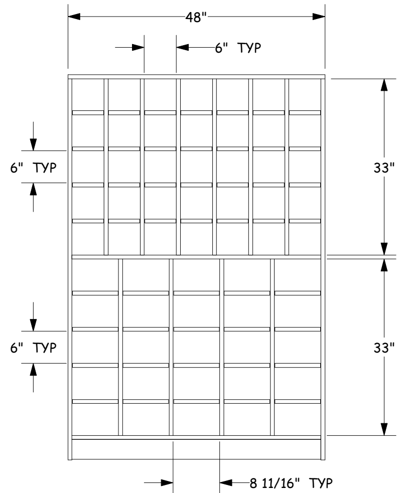
Front View (Shown Without Doors)
